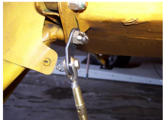
Figure 5 - Rear Two-Hole Tang Installation
